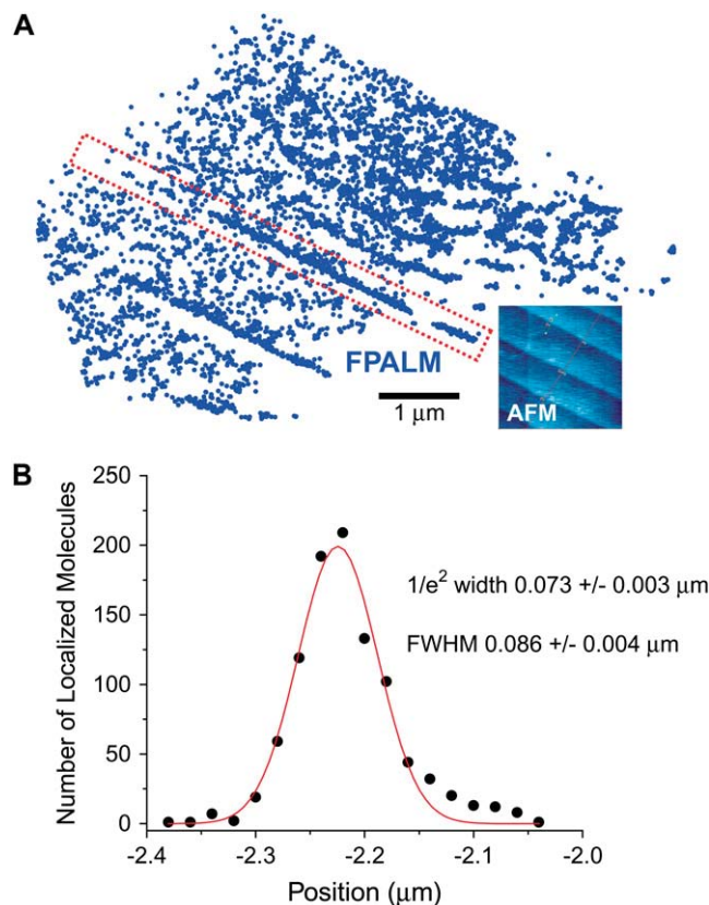
FIGURE 8 FPALM image of an R-cut single-crystal wafer of sapphire annealed at high temperature to produce atomic terraces, labeled with PA-GFP. (A) The positions of PA-GFP molecules localized over a period of 500 s are plotted (blue points) and compared with an atomic force microscope (AFM) image (inset) of the same sample (not necessarily the same area). Atomic step dislocations spaced laterally by 200–630 nm are visible by both techniques, because the PA-GFP has localized to those dislocations upon drying. Scale bar ( 1 \mu\text{m} ) applies to both the FPALM and the AFM images. Note the gradient in particle density across the dislocations shown by FPALM. The red dotted box corresponds to the profile in B. (B) Analysis of the profile of a dislocation. The histogram of molecular positions (black points) as a function of distance perpendicular to the dislocation reveals the width of the feature as visualized by FPALM. Fitting the profile with a Gaussian (red line) yielded a 1/e^2 half-width of 73 \pm 3 nm, and an FWHM of 86 \pm 4 nm.
